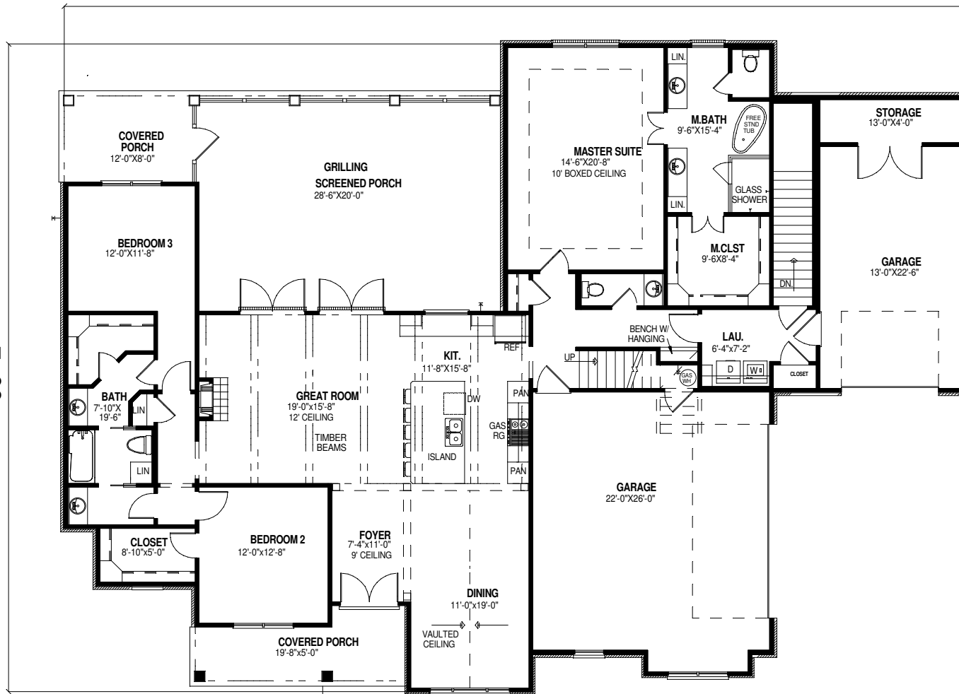
MEN5390-1 MAIN FLOOR CODY CREEK PLACE
